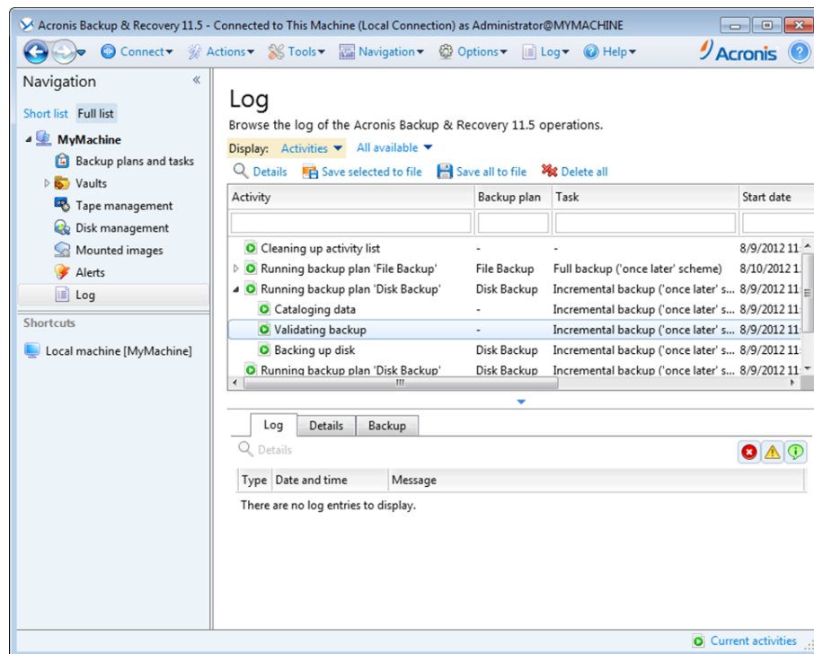
"Log" view
