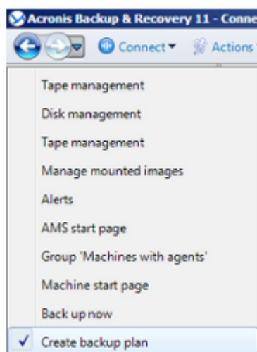
Navigation buttons
